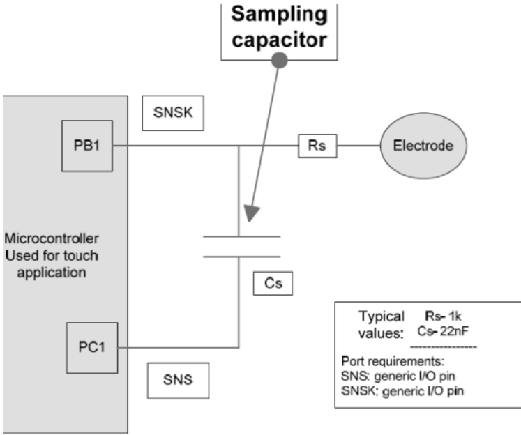
Rs- Series resistor, Cs – Sample capacitor, PB1- PortB bit1, and PC1- PortC bit1
